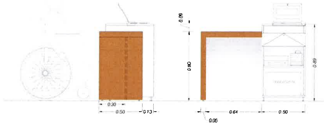
ELEVATIONS
