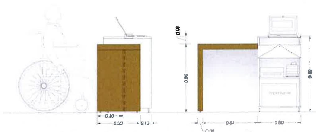
ELEVATIONS
