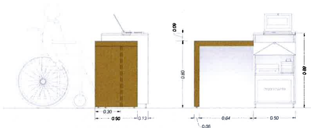
ELEVATIONS
