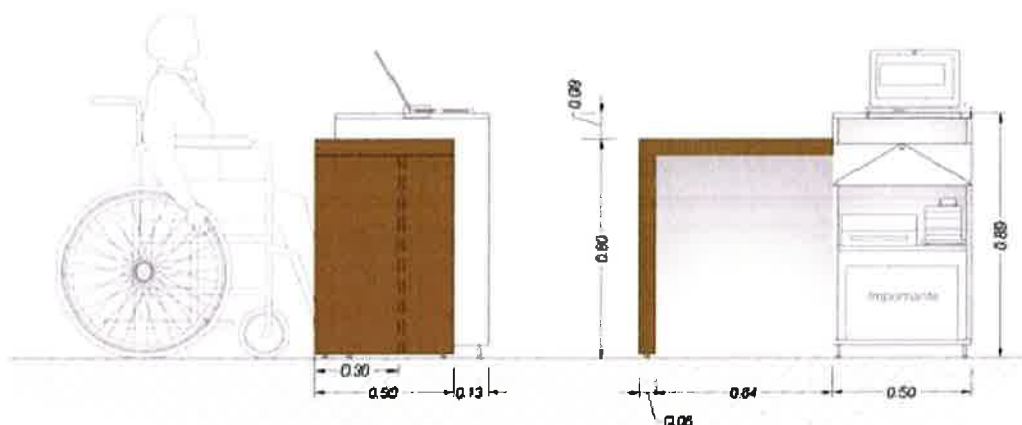
ELEVATIONS
