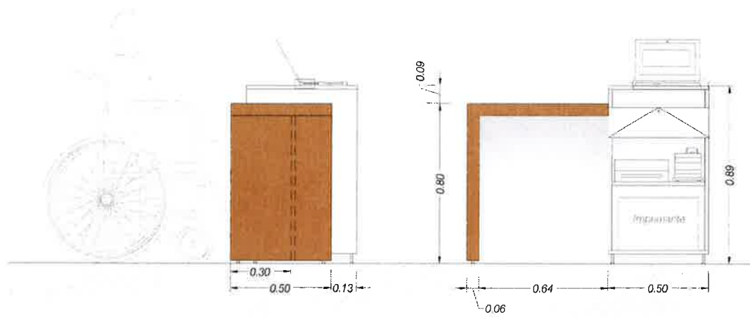
ELEVATIONS
