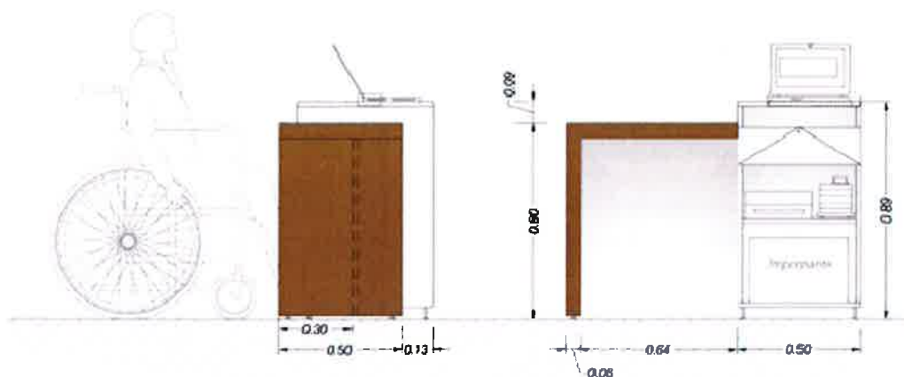
ELEVATIONS
